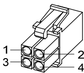
40/60/80电机电源插头
